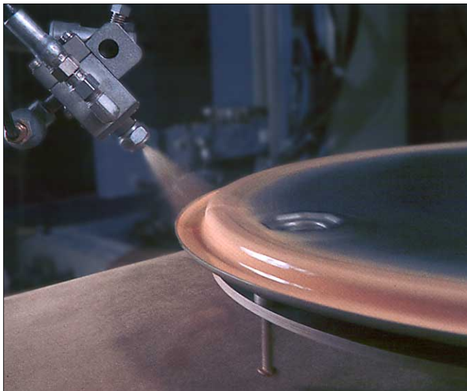
A7A guns are used on high-speed drum painting lines to deliver fast, precise coating coverage.
